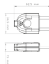
male plugs enchufes machos
